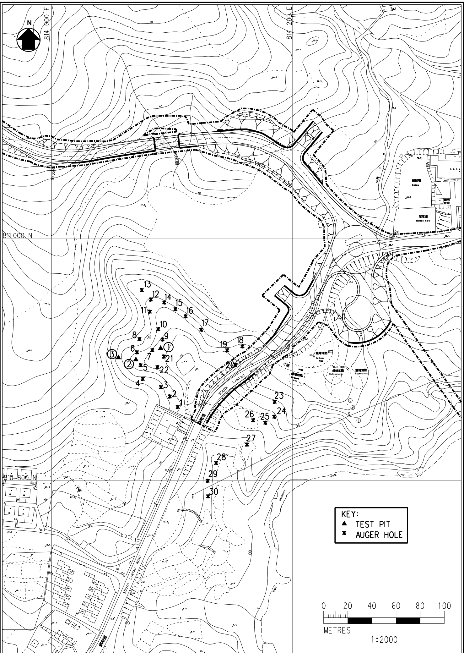
LOCATION OF AUGER HOLES AND TEST PITS 1,2, AND 3 IN CHEUNG SHA (AREA 2)
